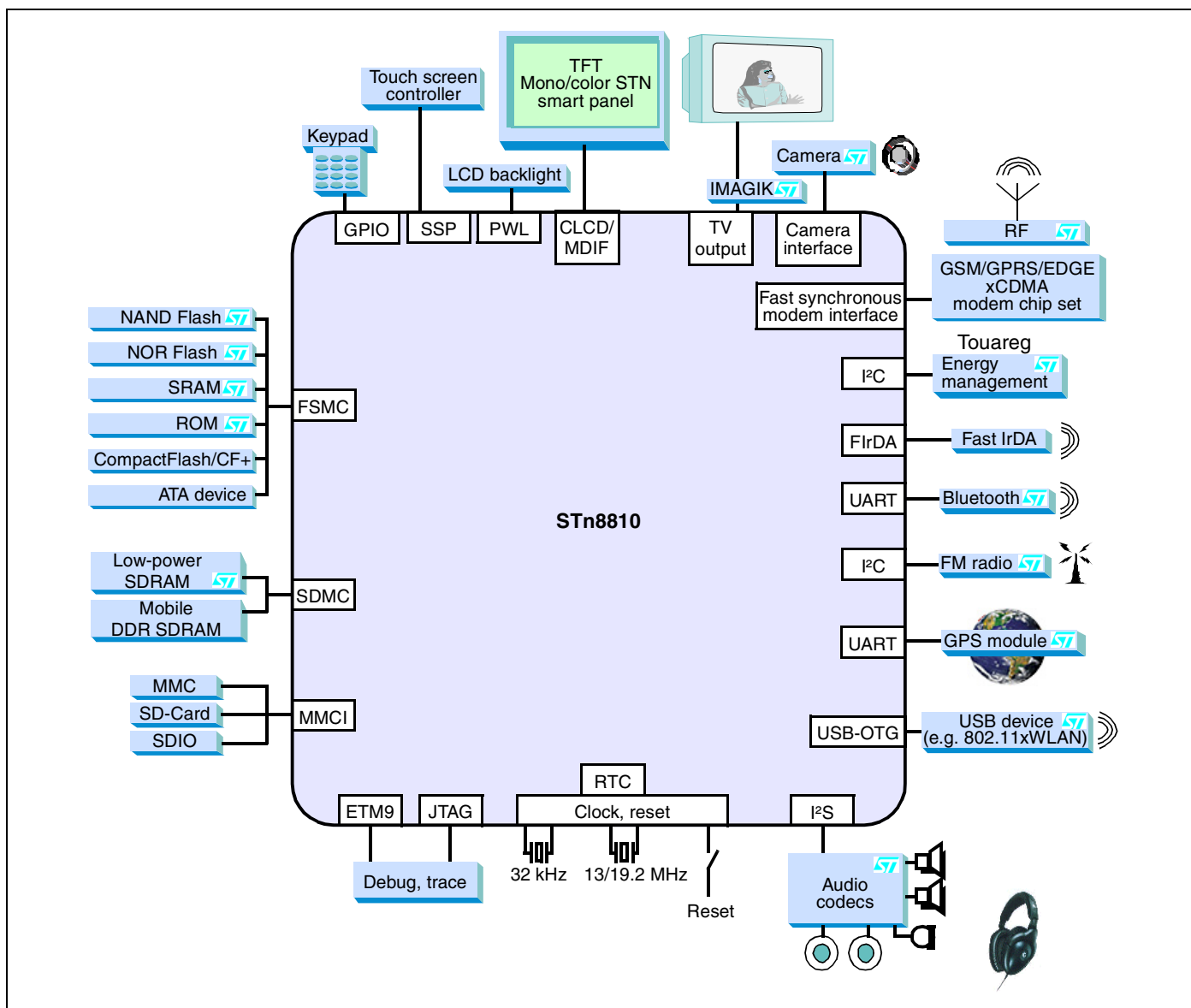
Figure 1: Typical system architecture using the STn8810
