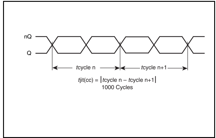
Cycle-to-Cycle Jitter
