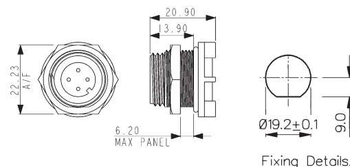
Fixing Details.
