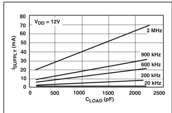
FIGURE 2-12: Supply Current vs. Capacitive Load.
