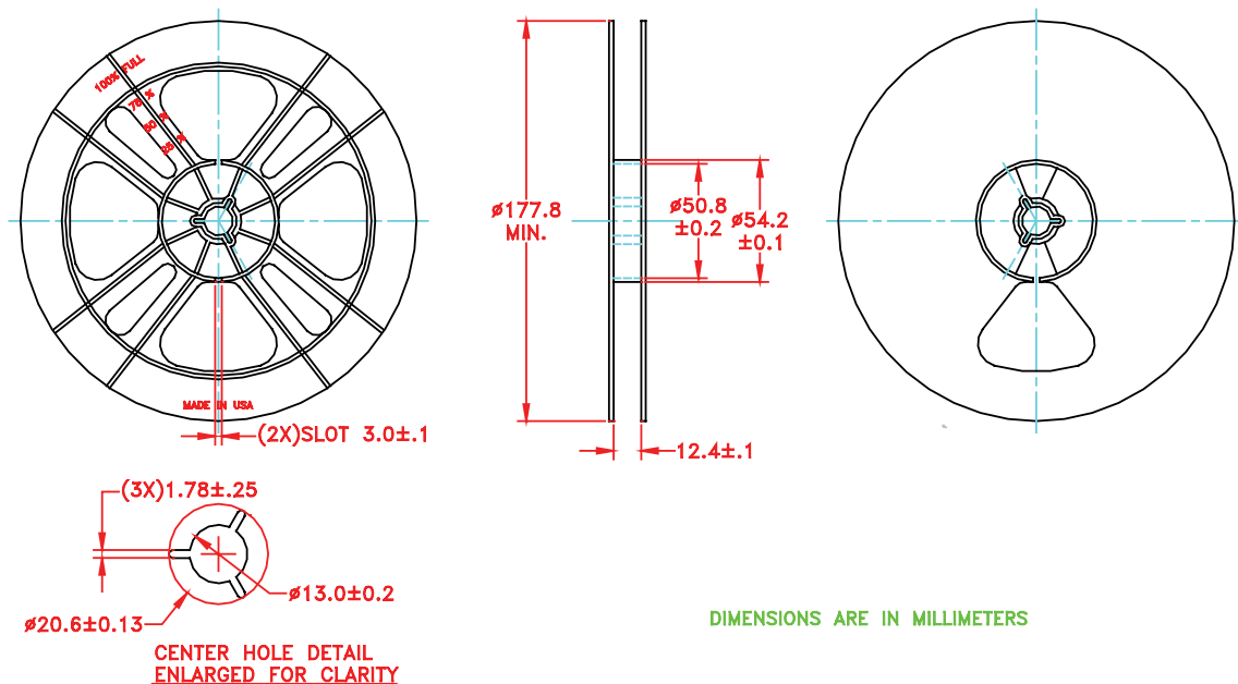
Figure 8: Carrier Tape
