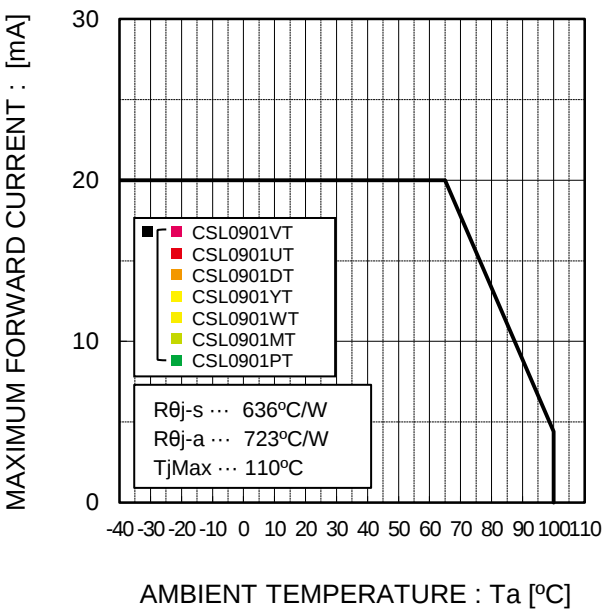
Fig.3 Derating
