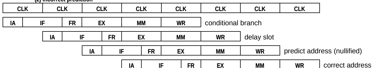
Figure 6.2 Pipeline operation for branch prediction.
