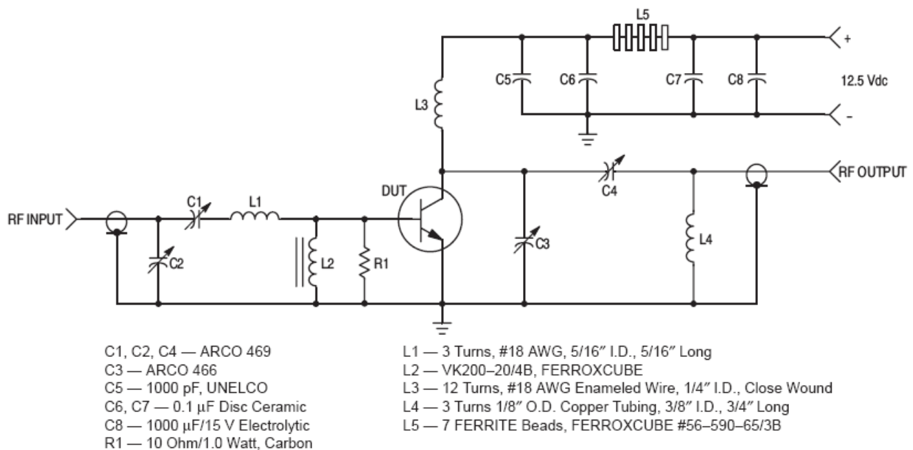
Figure 1. 30 MHz Test Circuit Schematic
