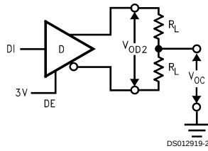
FIGURE 1. V_{OD}
