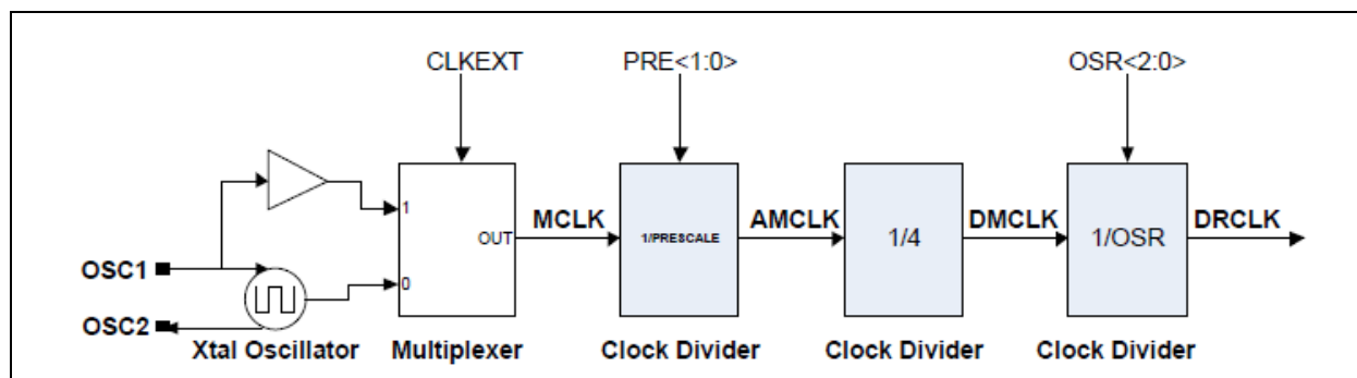
FIGURE 4-1: Clock Sub-Circuitry.
