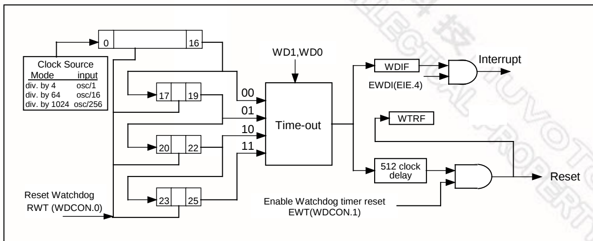
Figure 19. Watchdog Timer
