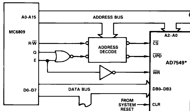
Figure 8. AD7549-MC6809 Interface
