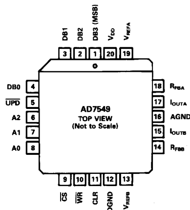
PLCC
