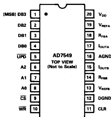
DIP
