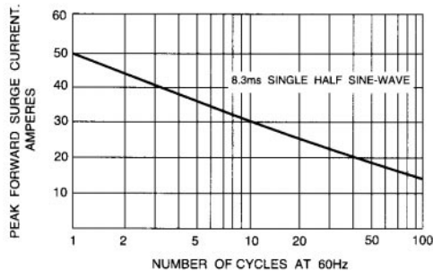
FIG. 3 - MAXIMUM FORWARD SURGE CURRENT
