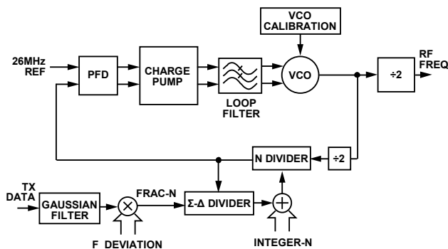
Figure 78. RF Frequency Synthesizer Architecture
