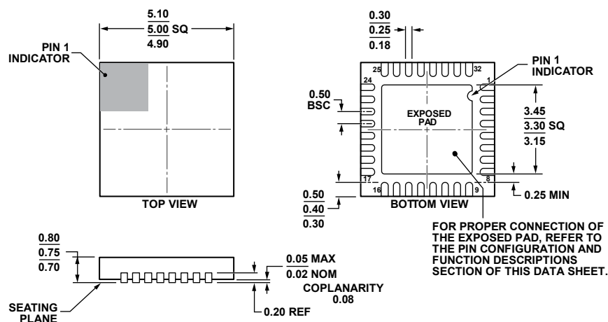
Figure 88. 32-Lead Lead Frame Chip Scale Package [LFCSP_WQ]
