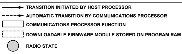
Figure 47. Radio State Diagram
