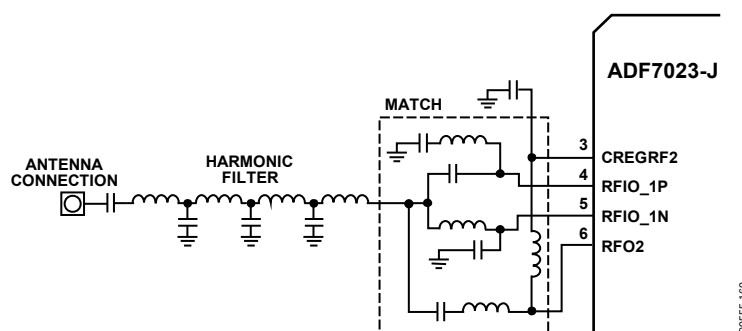
Figure 85. Combined Single-Ended PA and LNA Match
