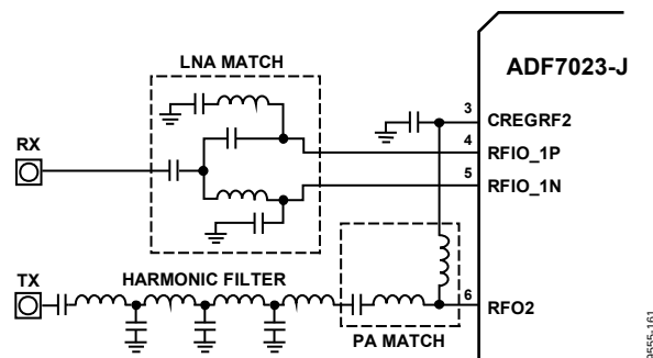
Figure 84. Separate Single-Ended PA and LNA Match
