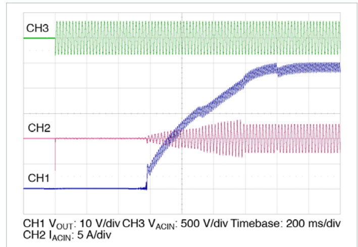
Figure 8 — Typical startup waveform, application of V_{IN} , I_{OUT} = 8.3\text{ A} , C_{OUT} = 10,000\text{ }\mu\text{F}
