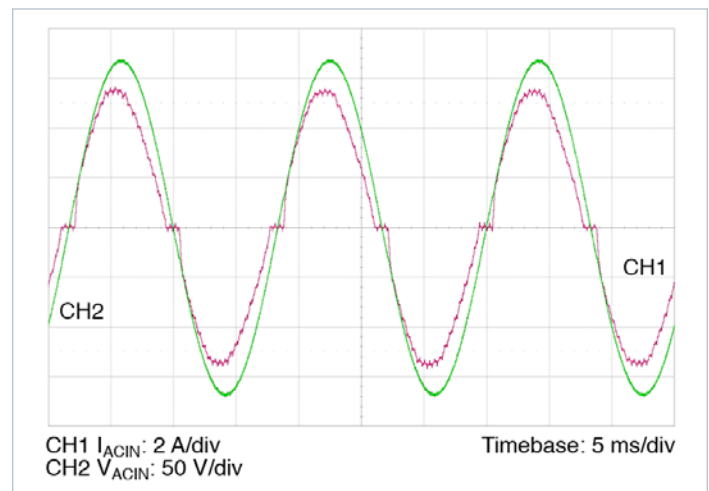
Figure 12 — Typical line current waveform, V_{IN} = 120\text{ V} , 60 HZ I_{OUT} = 8.3\text{ A} , C_{OUT} = 10,000\text{ }\mu\text{F}
