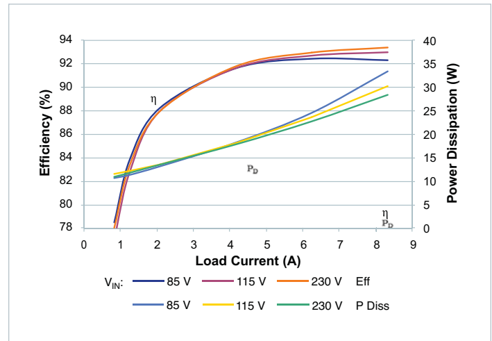
Figure 16 — V_{IN} to V_{OUT} efficiency and power dissipation vs. V_{IN} and I_{OUT} , T_{CASE} = 20^\circ C
