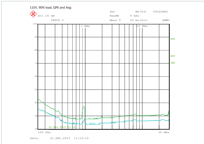
Figure 13 — Typical EMI Spectrum, Peak Scan, 90% load, 115 V_{IN} , C_{OUT} = 10,000 \mu F using Typical Chassis Mount Application Circuit
