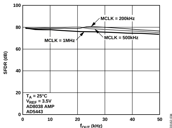
Figure 33. Wideband SFDR vs. f_{OUT} Frequency (AD5443)
