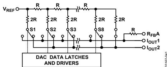
Figure 40. Simplified Ladder
