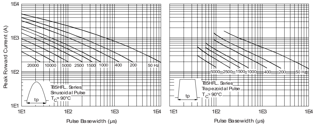
Fig. 44 - Frequency Characteristics
