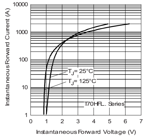
Fig. 47 - Forward Voltage Drop Characteristics
