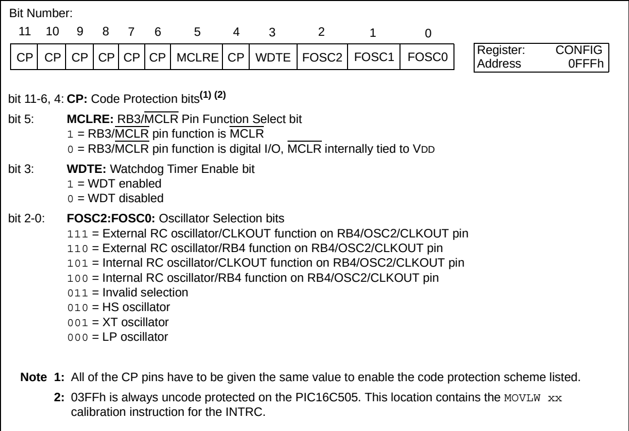
FIGURE 3-1: CONFIGURATION WORD BIT MAP
