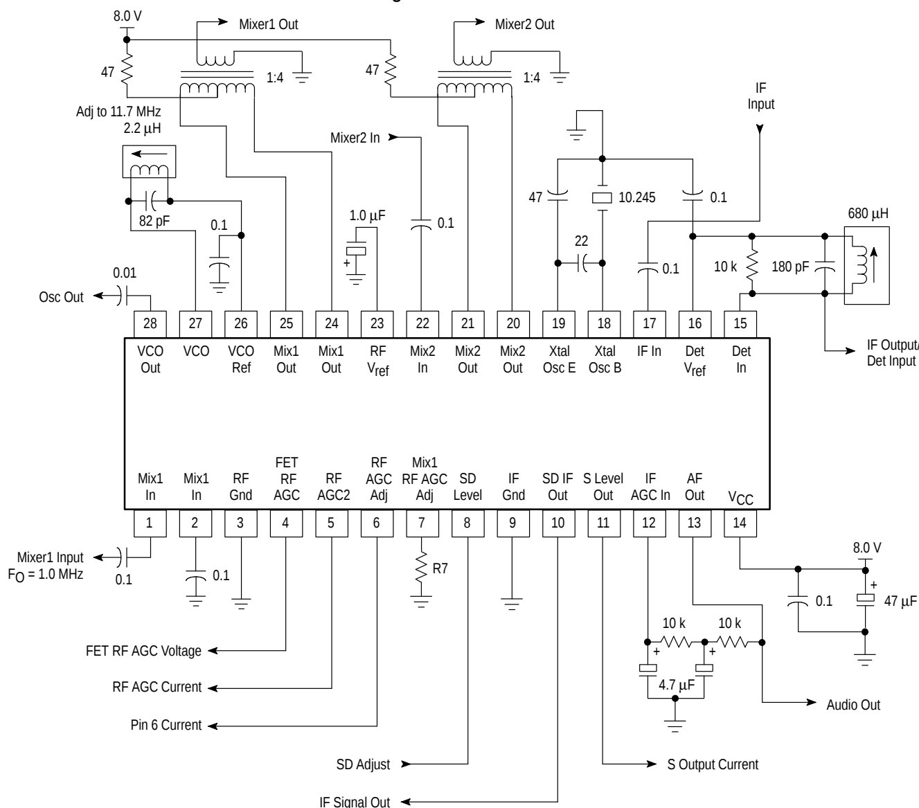
Figure 1. Test Circuit
