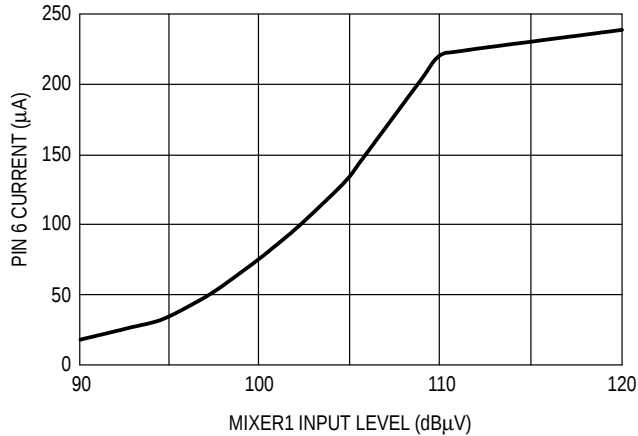
Figure 6. Pin 6 Current versus Mixer1 Input Level
