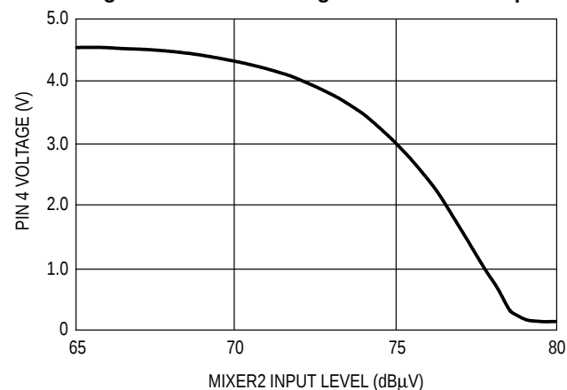
Figure 5. RF AGC Voltage versus Mixer2 Input
