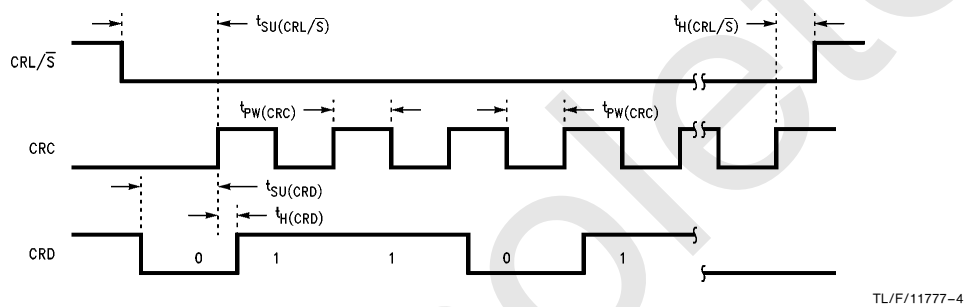
FIGURE 4. MICROWIRE™ Compatible Control Register Serial Load Timing Diagram
