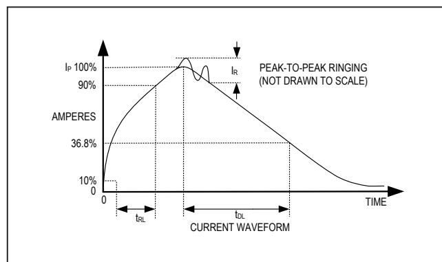
Figure 9. Human Body Current Waveform
