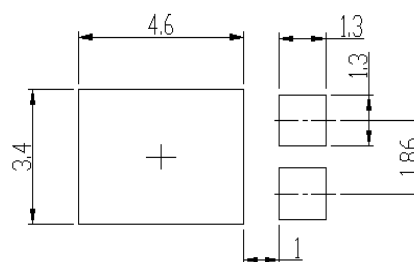
Soldering footprint
