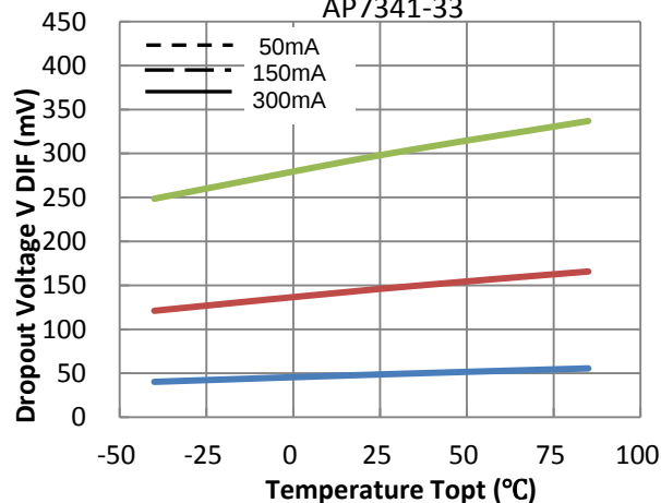
Dropout Voltage vs. Temperature AP7341-33
