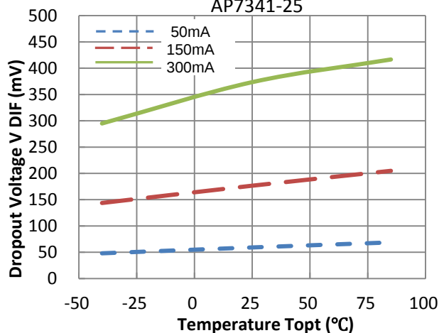
Dropout Voltage vs. Temperature AP7341-25
