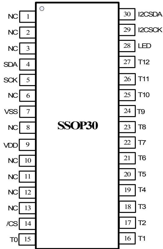
GPM8F377A Package
