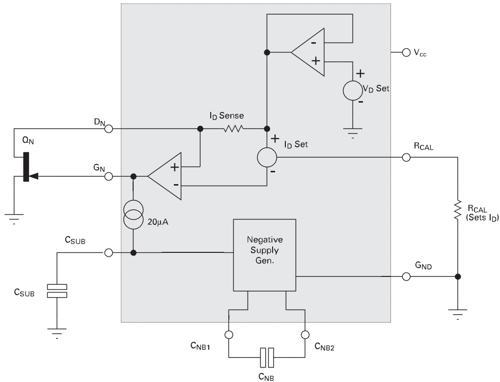
FUNCTIONAL DIAGRAM
