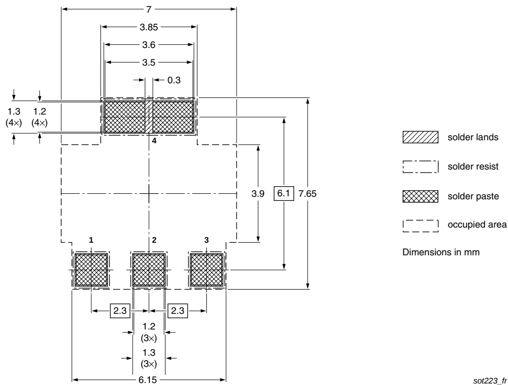
Fig 17. Reflow soldering footprint for SOT223 (SOT223)
