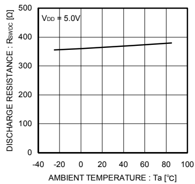
Fig.19 Switch discharge resistance
