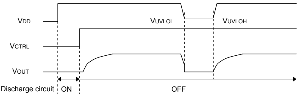
Fig.62 UVLO operation
