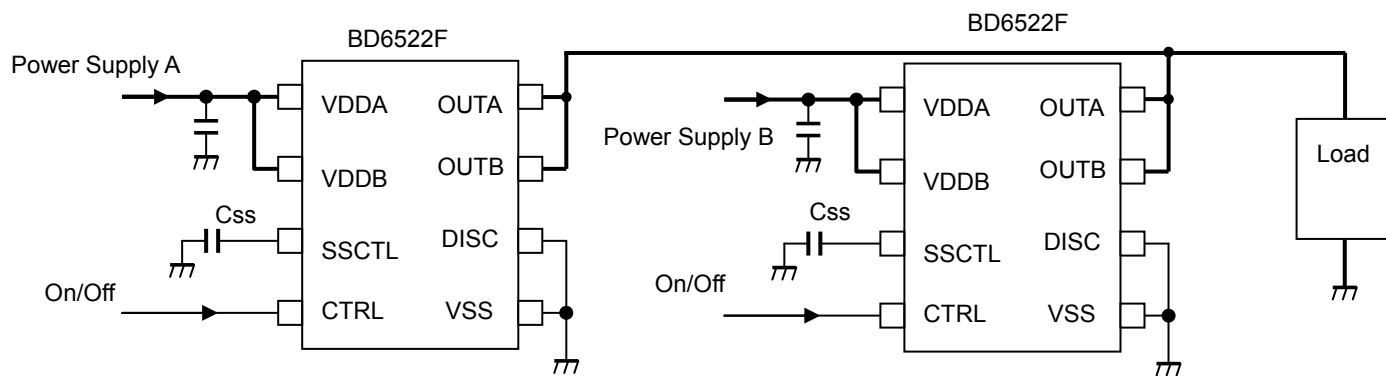
Fig.66 2 power supply changeover switch circuit (BD6522F)
