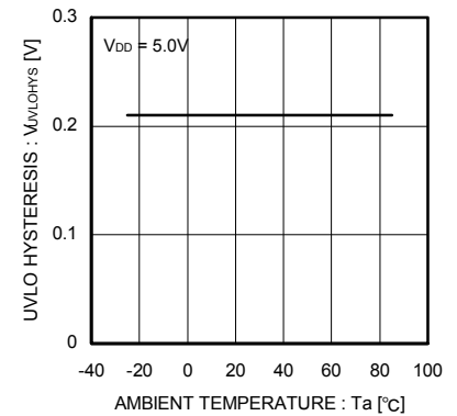
Fig.43 UVLO hysteresis voltage
