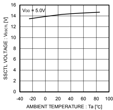
Fig.25 SSCTL output voltage
