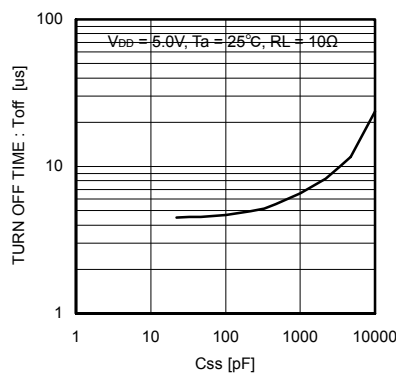
Fig.45 Turn Off time (vs. Ciss)
