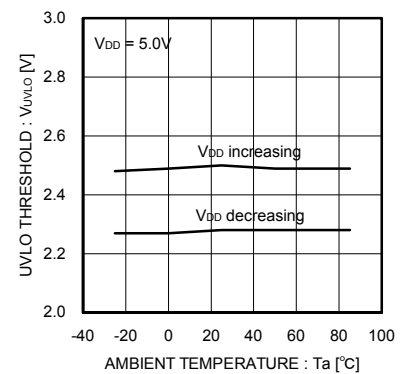
Fig.20 UVLO threshold voltage
