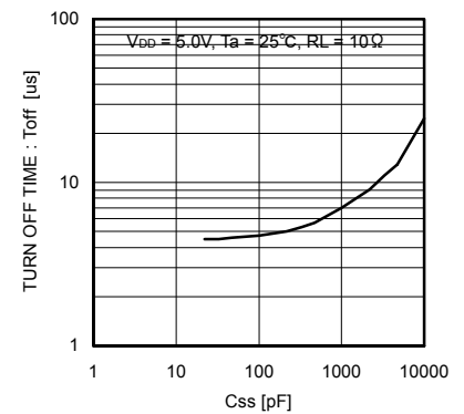
Fig.23 Turn Off Fall time (vs. Ccss)
