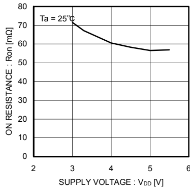
Fig.26 ON resistance
