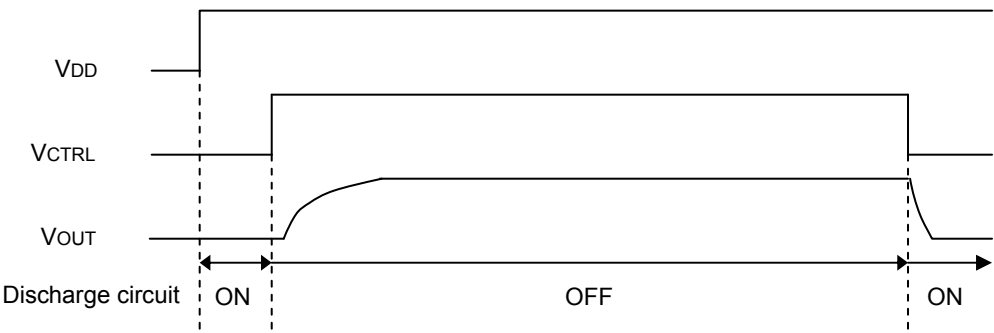
Fig.61 Normal operation
