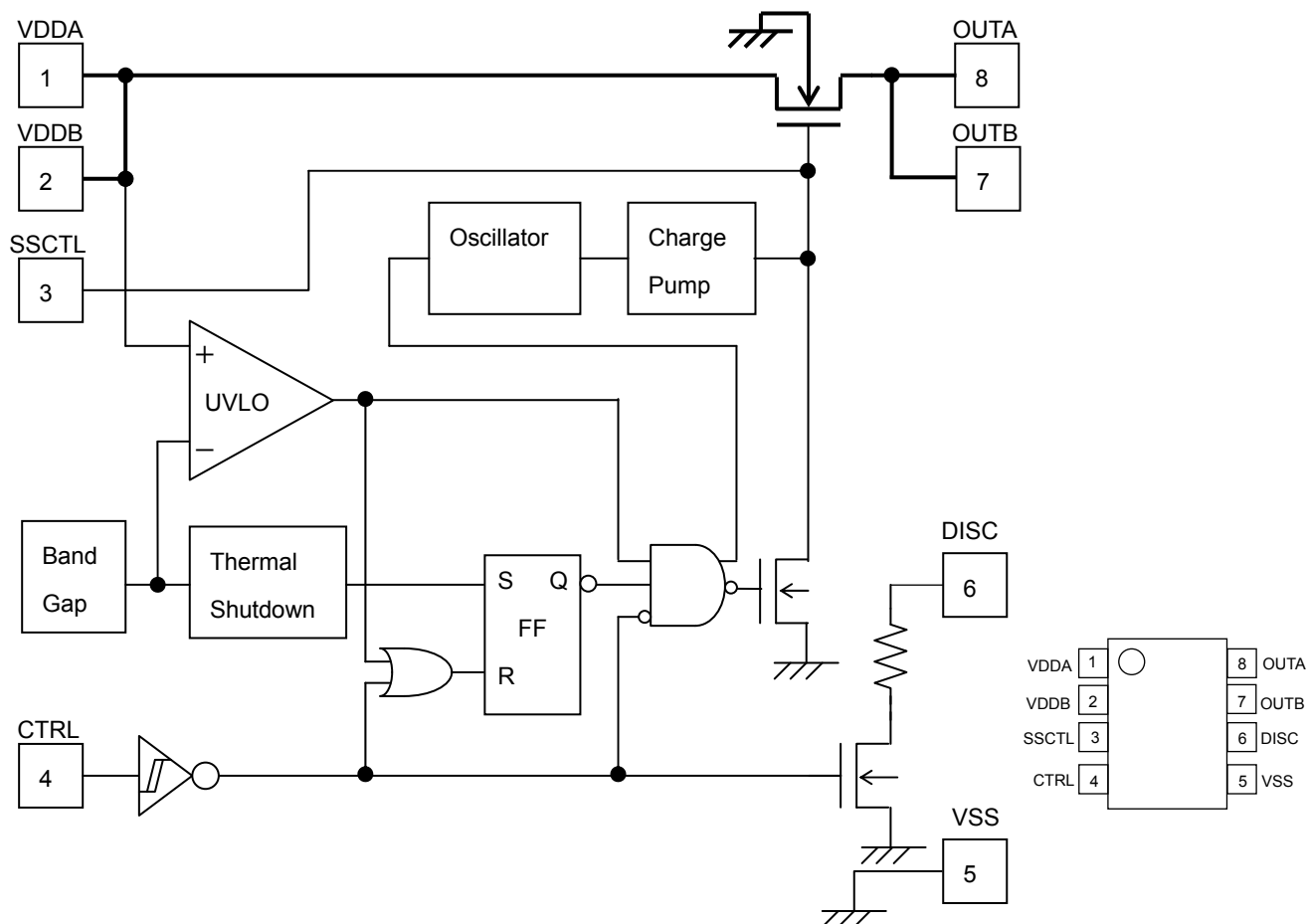
Fig.59 Block diagram(BD6522F)
