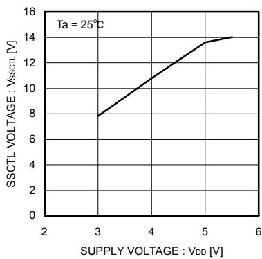
Fig.24 SSCTL output voltage
