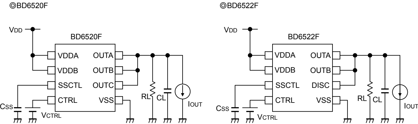
Fig.1 Measurement circuit
