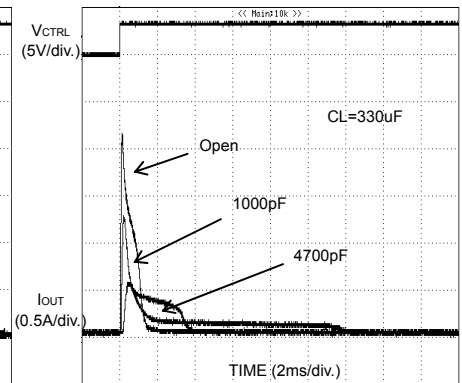
Fig.53 Inrush current vs. C_{SS} (BD6522F)
