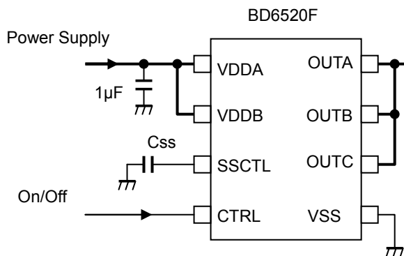
Fig.64 Power supply switch circuit (BD6520F)
