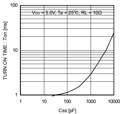
Fig.44 Turn On time (vs. Ciss)
