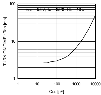
Fig.22 Turn On Rise time (vs. Ccss)
