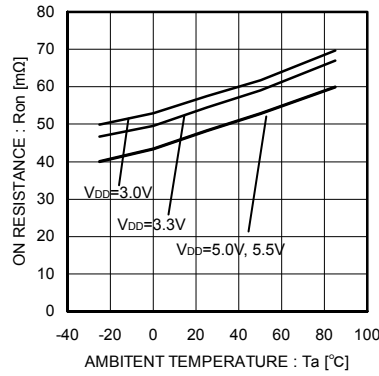
Fig.4 On resistance
