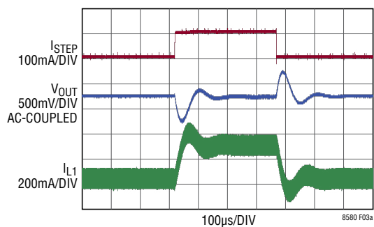
(3a) Transient Response Shows Excessive Ringing
