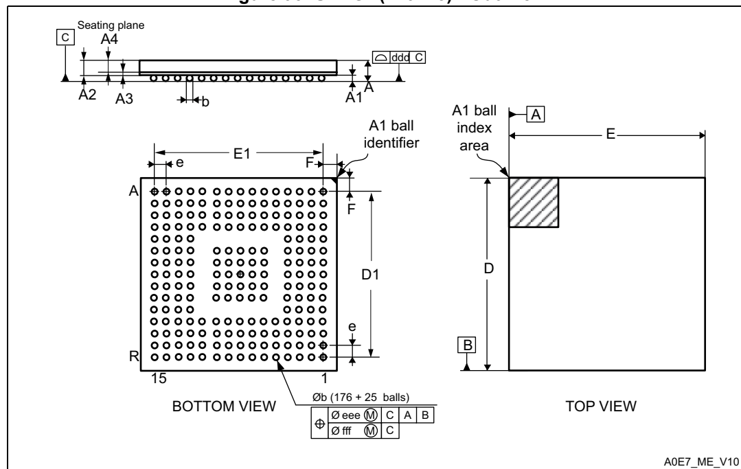
Figure 93. UFBGA(176+25) - Outline
