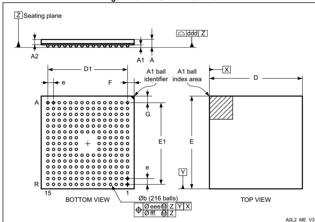
Figure 98. TFBGA216 - Outline
