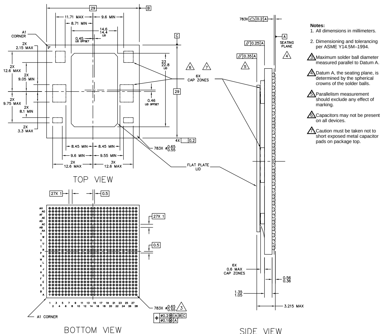
Figure 45. MSC8144EC Mechanical Information, 783-ball FC-PBGA Package
