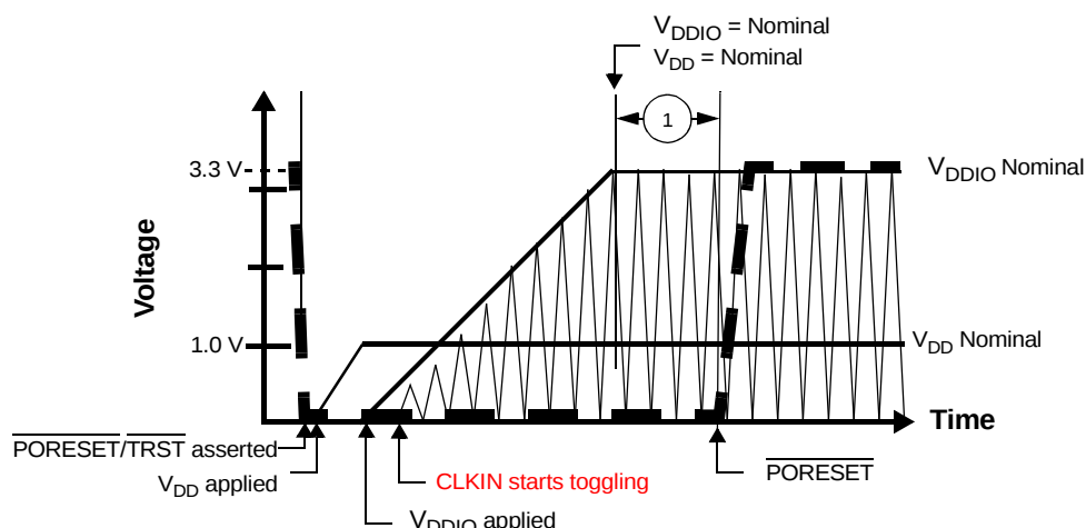
Figure 7. Start-Up Sequence with V_{\text{DD}} Raised Before V_{\text{DDIO}} with CLKIN Started with V_{\text{DDIO}}
