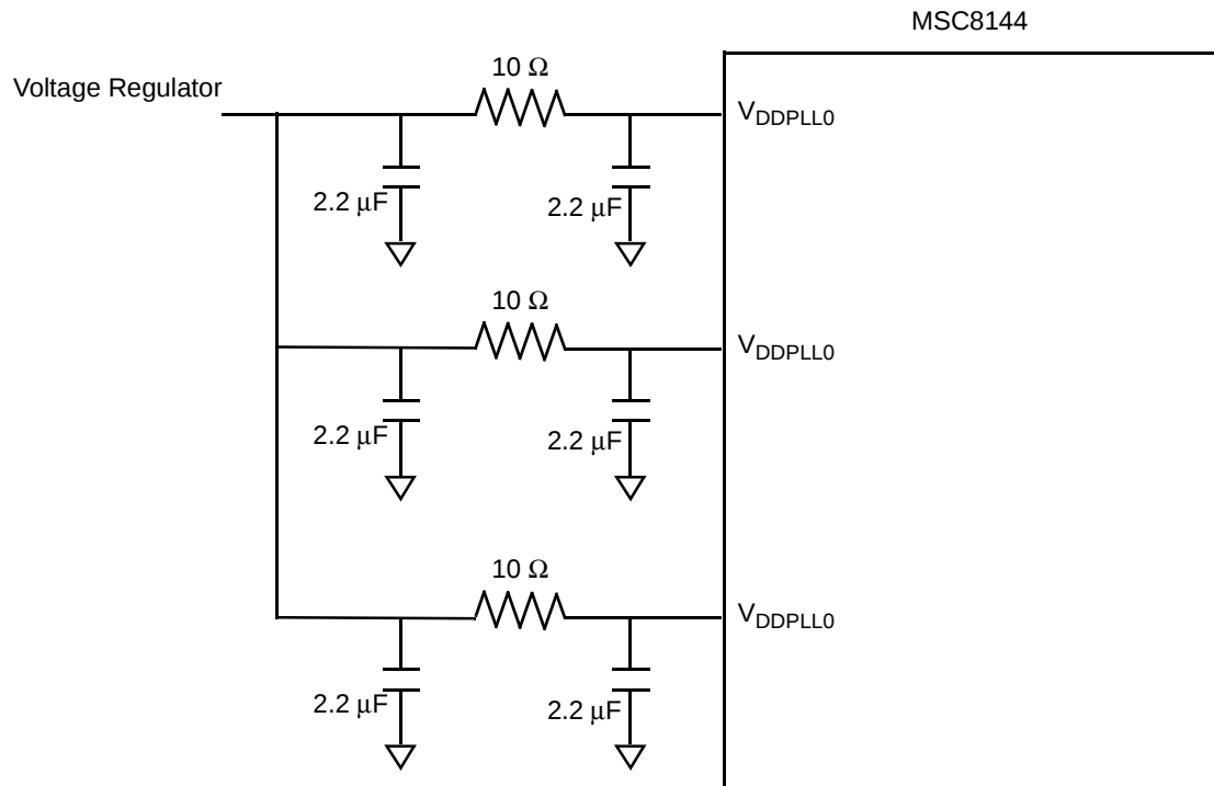
Figure 44. PLL Supplies
