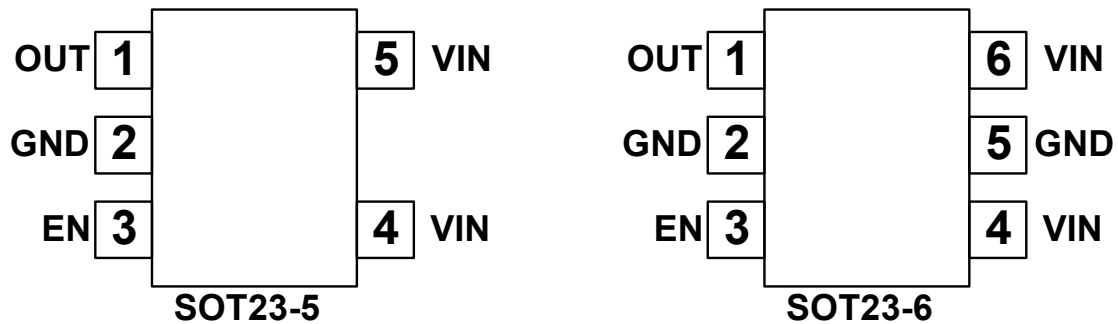
Figure 2: Pin Configuration
