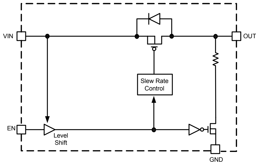
Figure 3: Function Block
