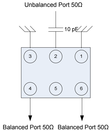
Schematic of BD0430J50100AHF with 10 pF capacitor on unbalanced port (pin #2)
