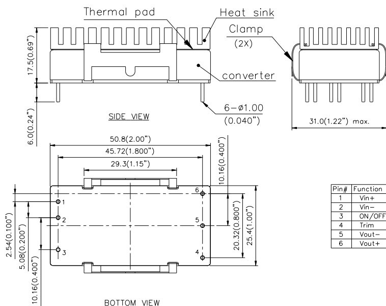
Mechanical Dimensions
