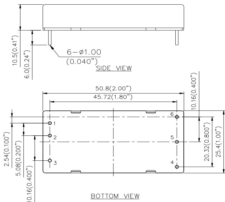
Mechanical Dimensions
