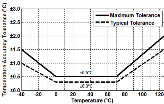
Figure 12. HS3004-ML1 Temperature Sensor Accuracy Tolerance
