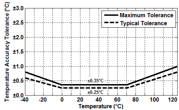
Figure 11. HS3003-ML1 Temperature Sensor Accuracy Tolerance
