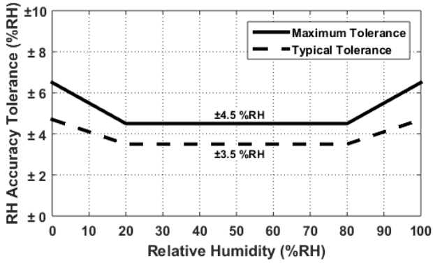
Figure 8. HS3004-ML1 RH Accuracy Tolerance at 25°C
