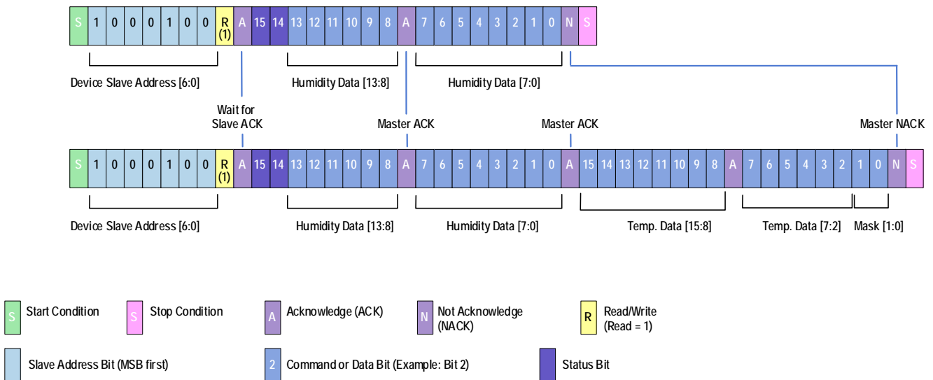
Figure 16. Data Fetch
