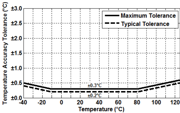
Figure 10. HS3001-ML1/HS3002-ML1 Temperature Sensor Accuracy Tolerance
