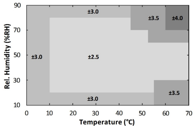
Figure 7. HS3003-ML1 RH Accuracy over Temperature
