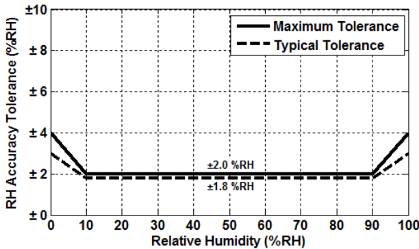
Figure 4. HS3002-ML1 RH Accuracy Tolerance at 25°C
