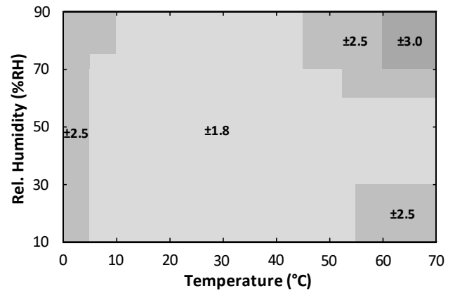
Figure 5. HS3002-ML1 RH Accuracy over Temperature
