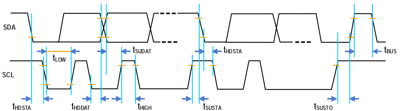
Figure 13. Timing Diagram
