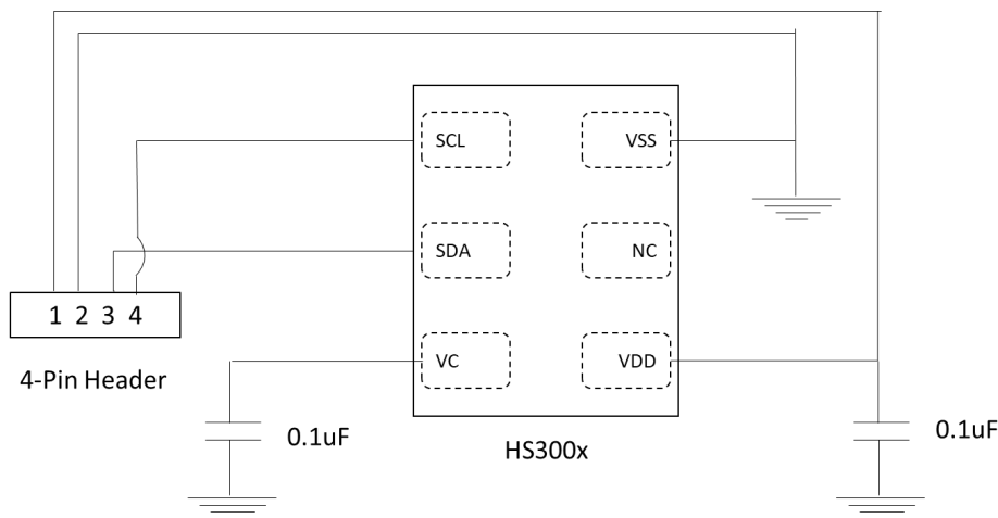
Figure 19. HS300x-ML1 Application Circuit
