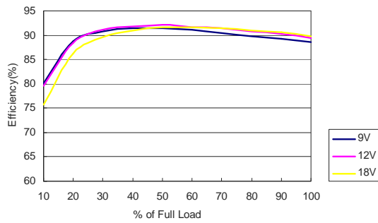
MKW50-12S033 Efficiency vs Load Current
