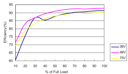
MKW50-48S05 Efficiency vs Load Current
