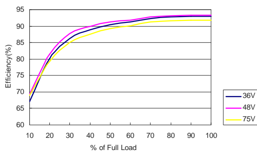
MKW50-48S033 Efficiency vs Load Current
