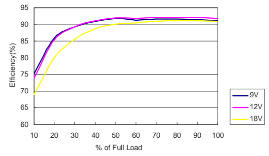
MKW50-12S05 Efficiency vs Load Current
