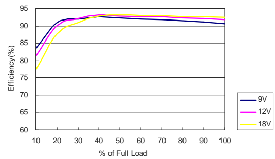
MKW50-12S12 Efficiency vs Load Current
