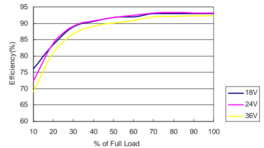
MKW50-24S033 Efficiency vs Load Current
