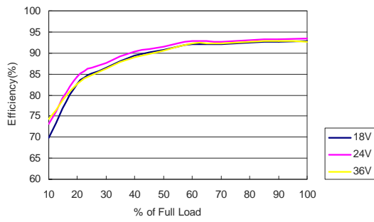
MKW50-24S15 Efficiency vs Load Current
