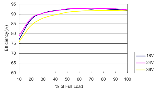
MKW50-12S24 Efficiency vs Load Current
