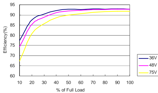
MKW50-48S12 Efficiency vs Load Current
