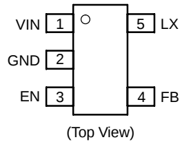
Figure 5. Pin Connections – TSOP5
