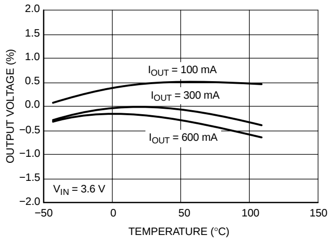
Figure 20. Output Voltage Accuracy ( V_{OUT} = 1.8 V)
