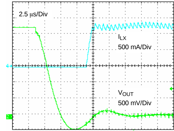
Figure 24. Short Circuit Protection ( V_{IN} = 3.6 V)
