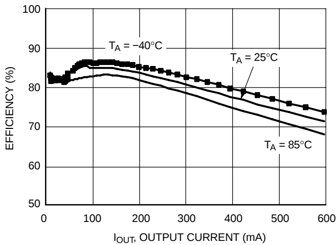
Figure 11. Efficiency vs. Output Current ( V_{OUT} = 0.9\text{ V} , V_{IN} = 3.6\text{ V} )
