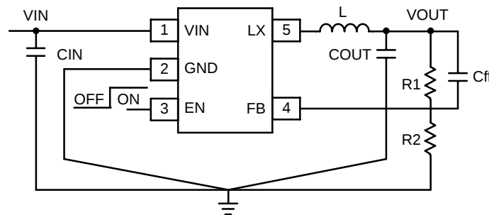
Figure 27. NCP1521 Board Schematic
