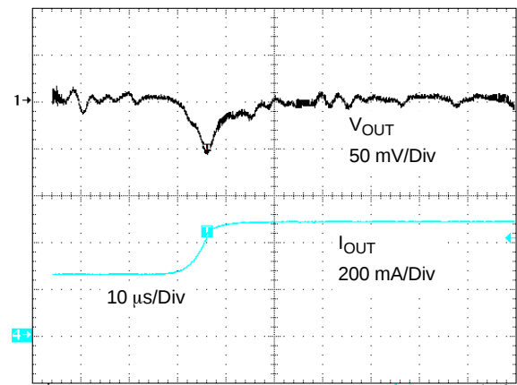
Figure 22. Load Transient Response in PWM Operation ( V_{IN} = 3.6 V)
