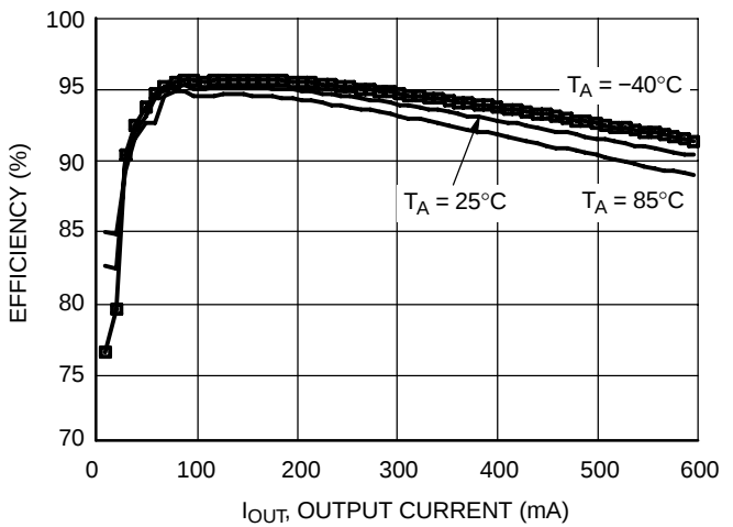
Figure 12. Efficiency vs. Output Current ( V_{OUT} = 3.3\text{ V} , V_{IN} = 4.5\text{ V} )
