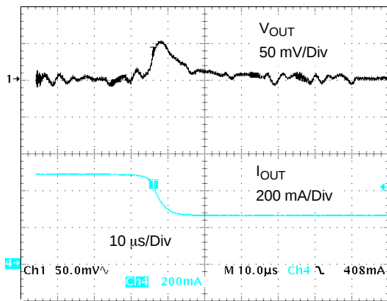
Figure 23. Load Transient Response in PWM Operation ( V_{IN} = 3.6 V)
