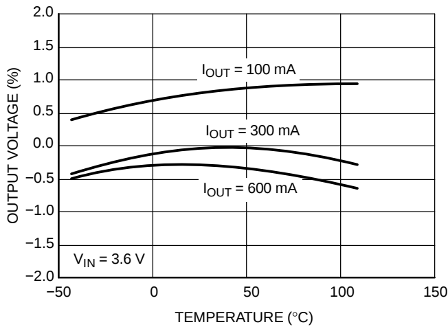
Figure 19. Output Voltage Accuracy ( V_{OUT} = 0.9 V)
