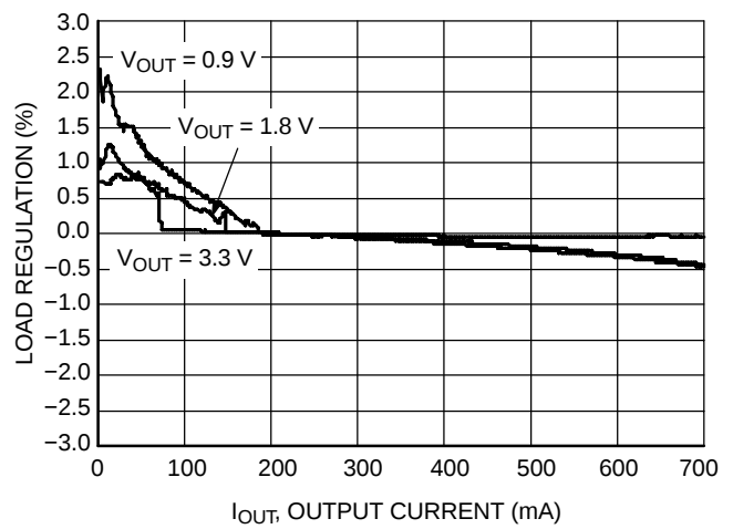
Figure 16. Load Regulation
