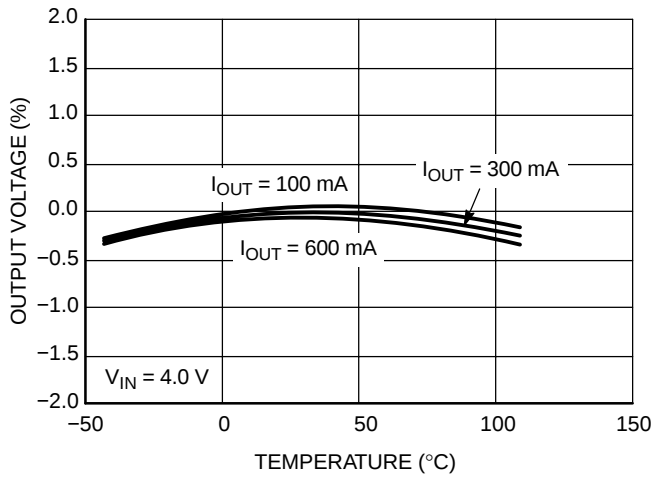
Figure 21. Output Voltage Accuracy ( V_{OUT} = 3.3 V)
