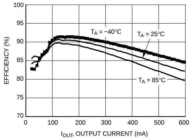
Figure 10. Efficiency vs. Output Current ( V_{OUT} = 1.8\text{ V} , V_{IN} = 3.6\text{ V} )
