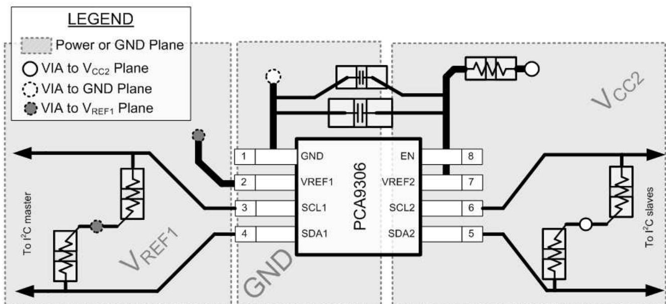
Figure 20. PCA9306 Layout Example
