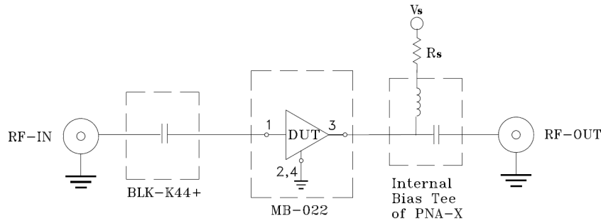
Fig 1. Characterization Circuit
