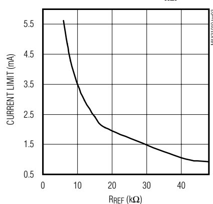
CURRENT LIMIT vs. R REF
