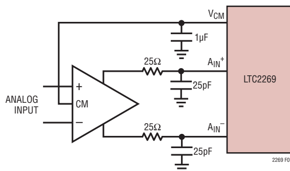
Figure 7. DC-Coupled Amplifier
