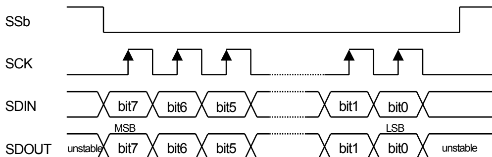
Fig. 7 4-Wire Serial Interface Timing
