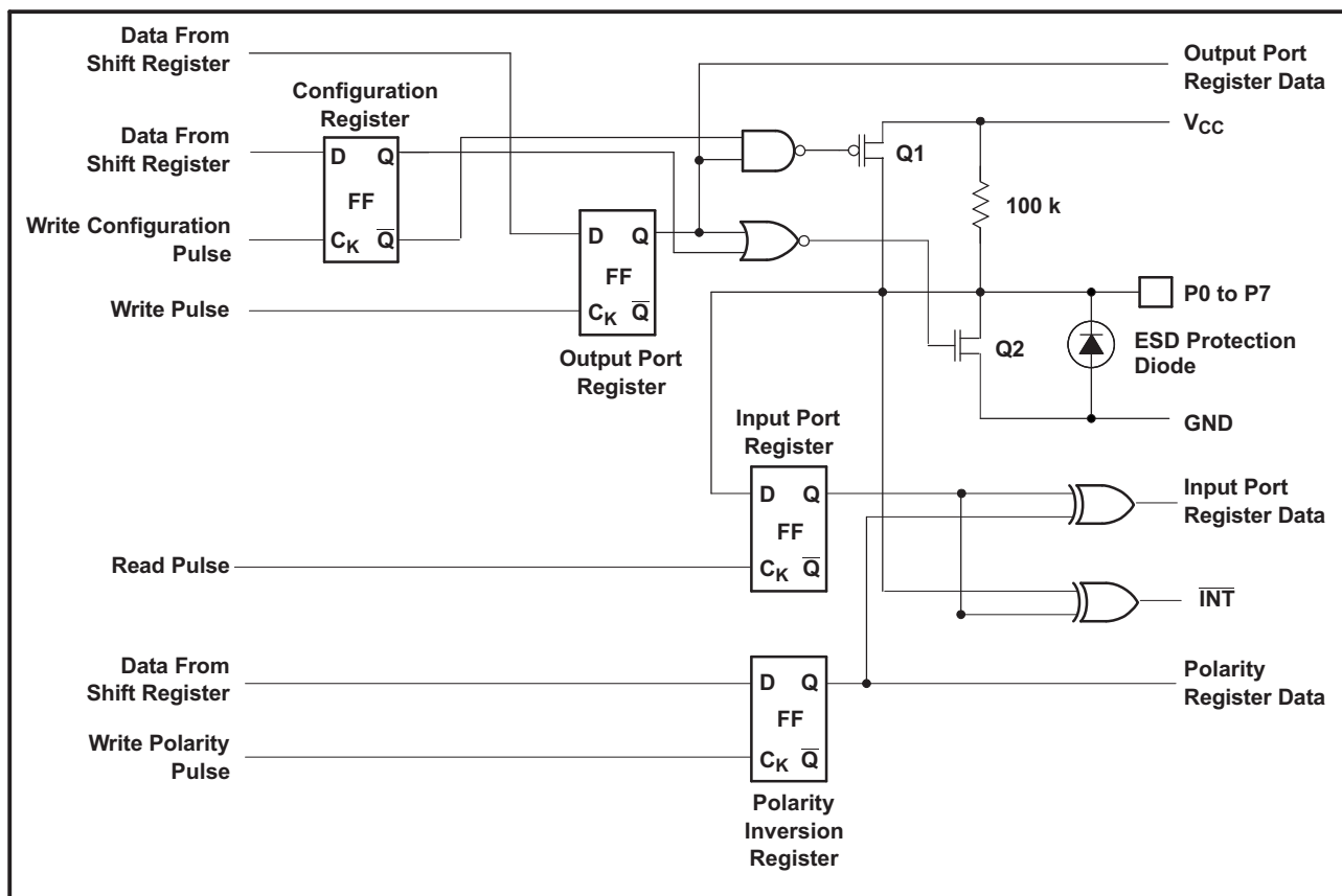
Figure 15. Simplified Schematic Of P0 To P7
