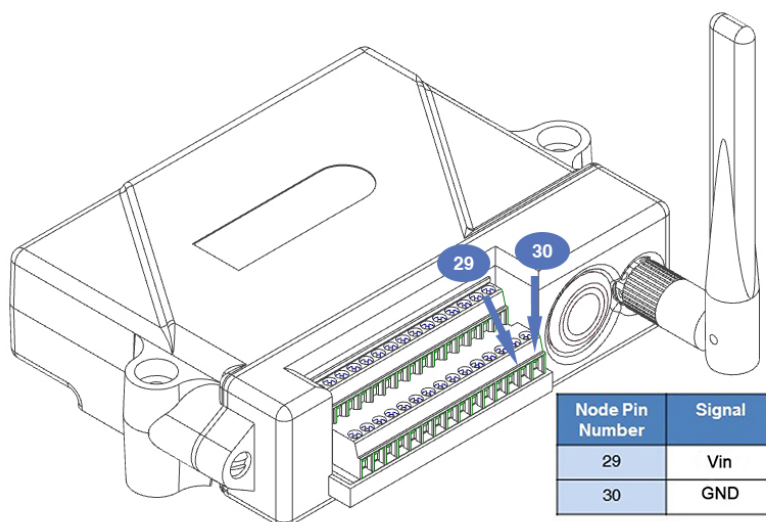
Figure 52 - External Power Connection
