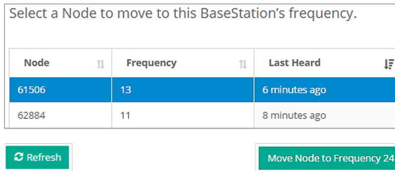
Figure 10 - Move Node
