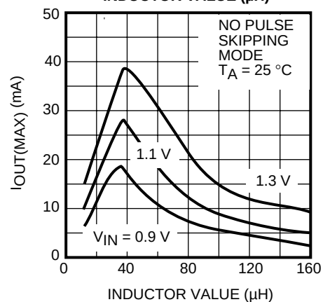
MAXIMUM OUTPUT CURRENT vs. INDUCTOR VALUE ( \mu H )
