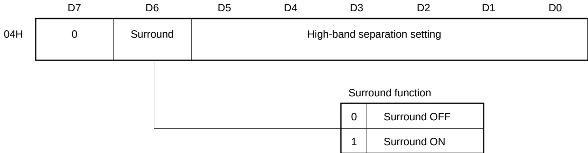
Figure 4-6. Surround Function
