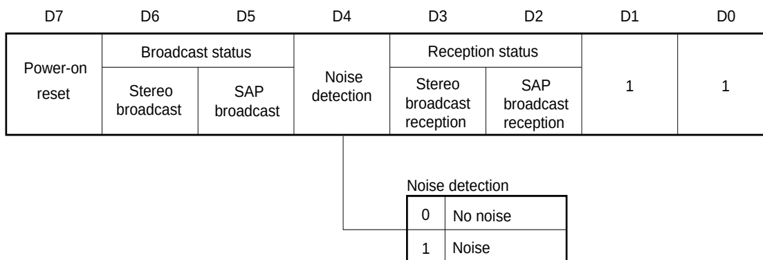
Figure 4-13. Noise Detection
