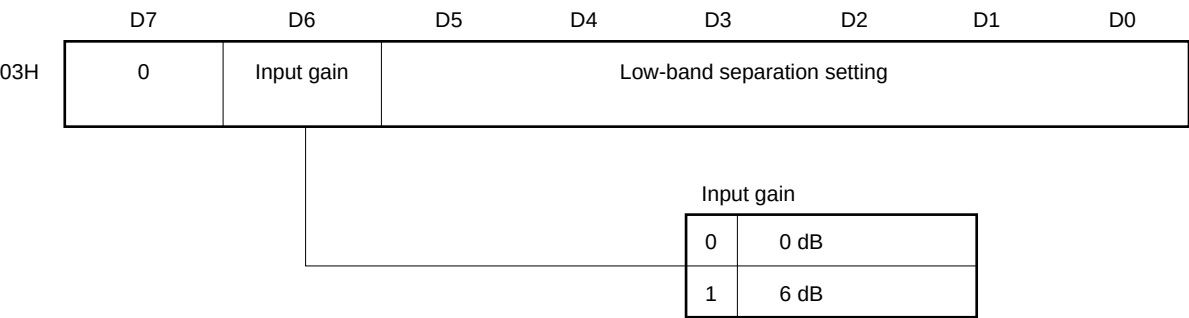
Figure 4-5. Input Gain
