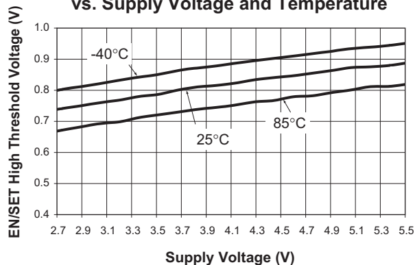
EN/SET High Threshold Voltage vs. Supply Voltage and Temperature
