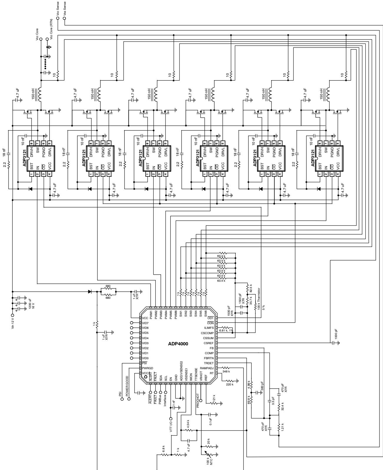
Figure 2. Application Schematic
