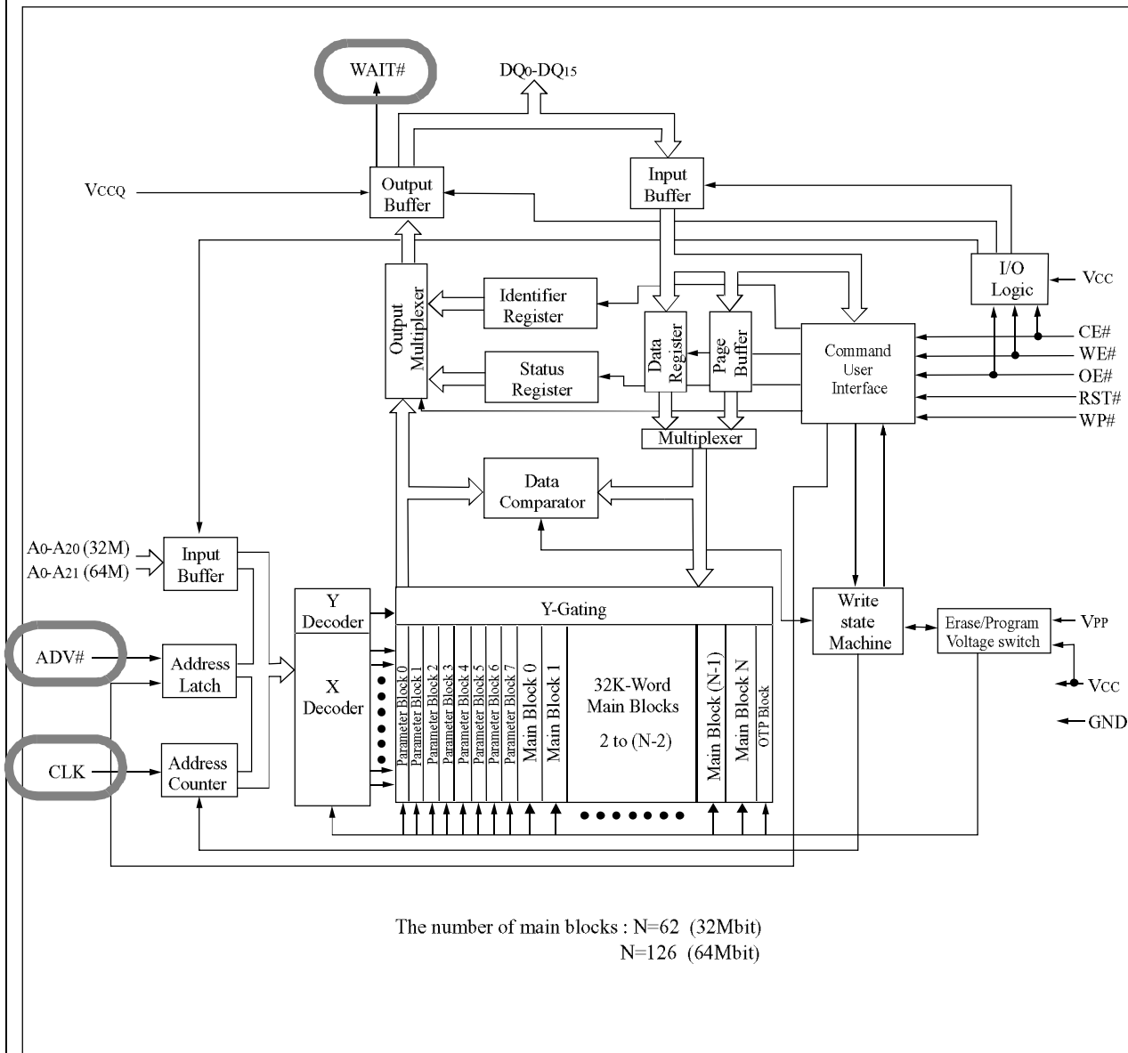
Figure 1. Block Diagram
