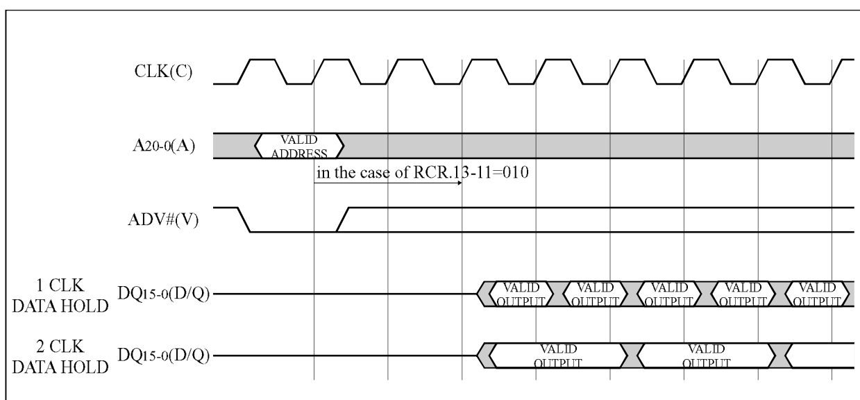
Figure 15. Output Configuration
