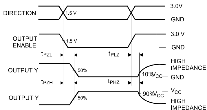
Figure 2. Switching Waveforms
