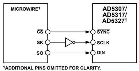
Figure 40. MICROWIRE-to-AD5307/AD5317/AD5327 Interface
